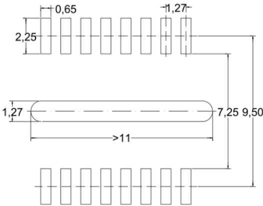
PCB Layout Reference View
